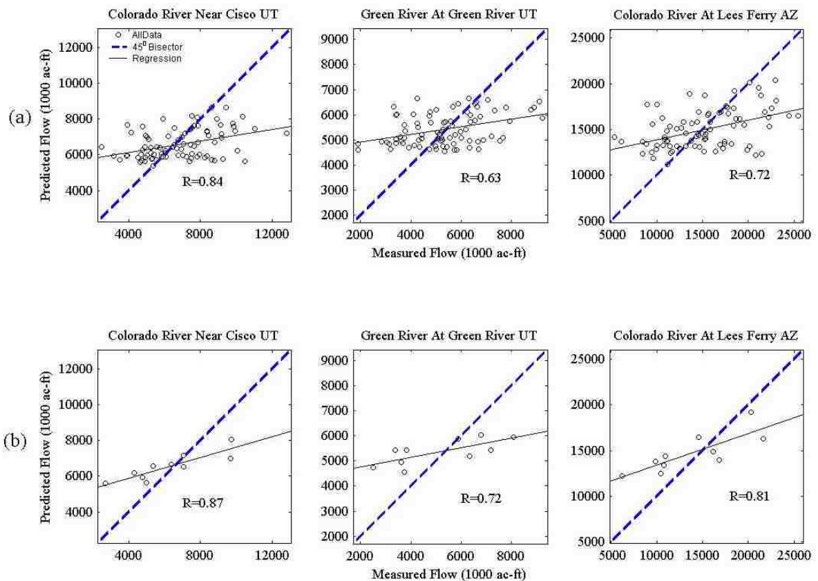
Figure 20: SVM predicted streamflow volumes at 't+3' for model I for (a) training phase and (b) testing phase at the three selected gages. Dashed line is the 45° bisector and solid line is true regression line between the measured and predicted streamflow volumes.
